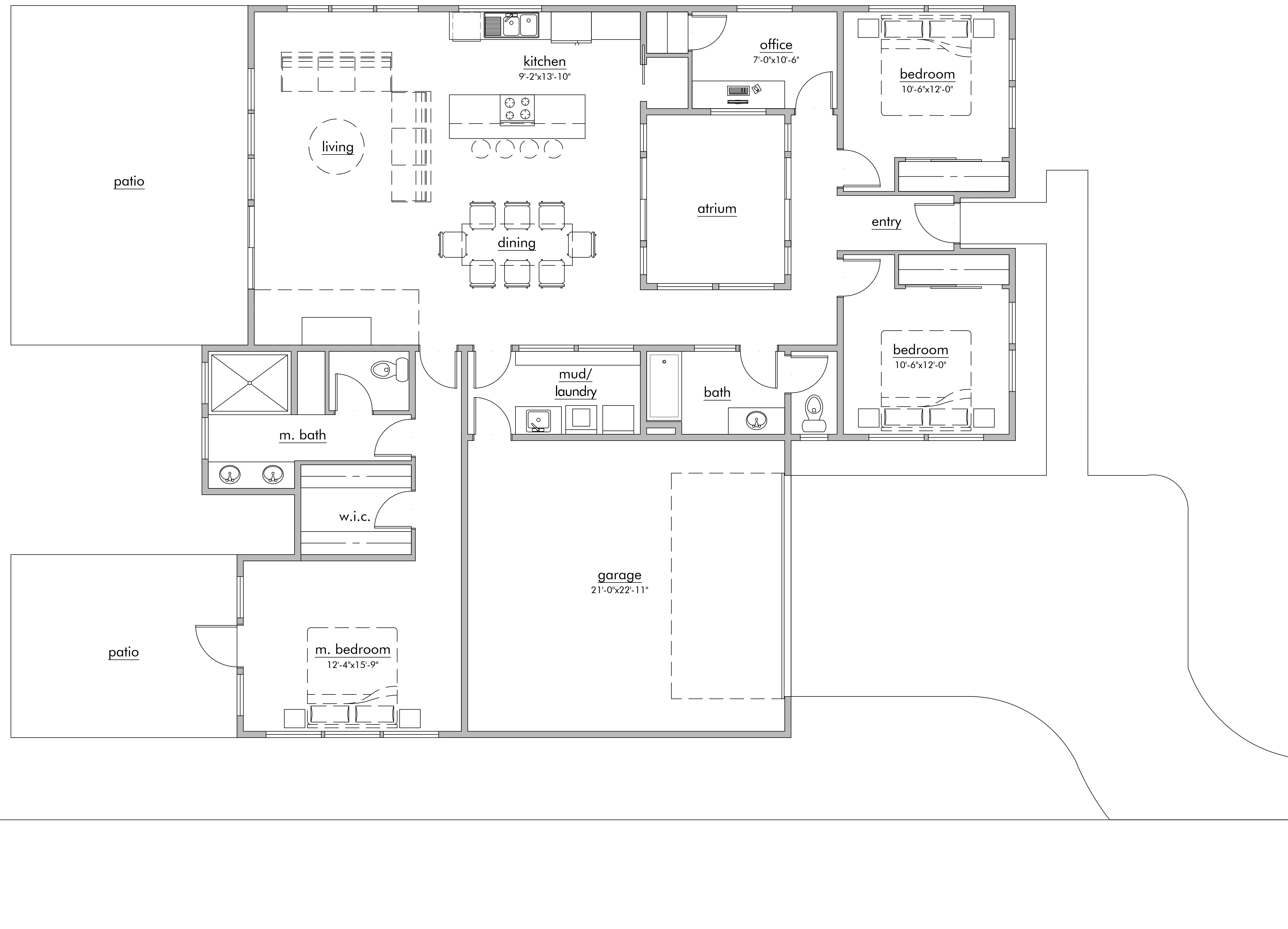
1 Hillview Parcel 1 Floor Plan 2109 s.f. Scale: 1/4" = 1'-0"
